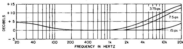
Typical recording (pre-equalization) for 1/4-inch tape recorders using NAB characteristics.
