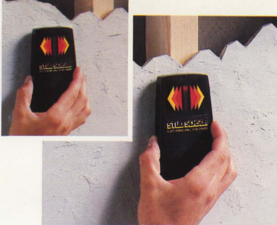
Stud Sensor "senses" density of wallboard. LED light signals change in mass as it passes over left edge of stud or joist. Once past stud, LED goes off indicating width of stud.
